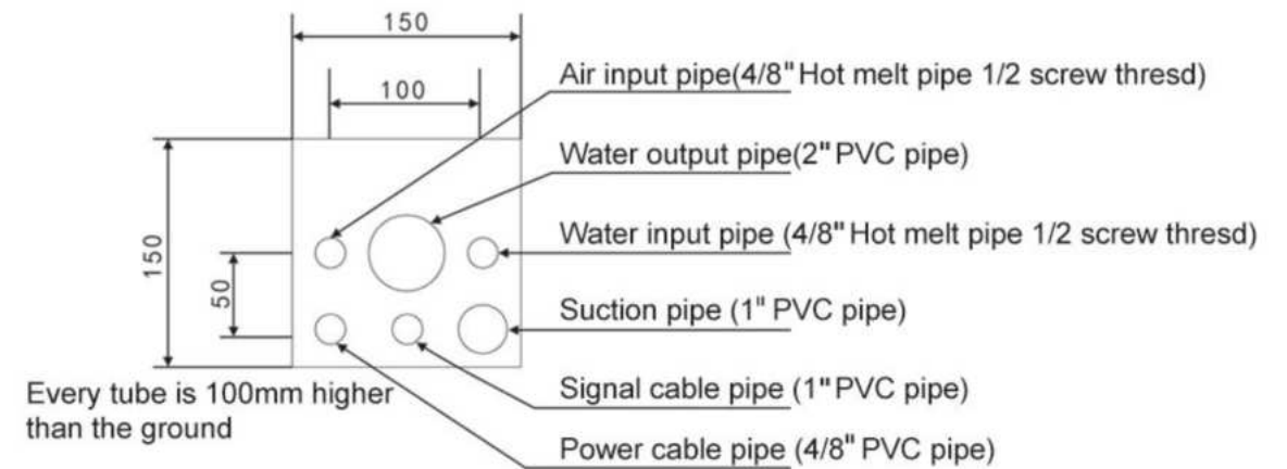
Pre-buried pipe distribution map
